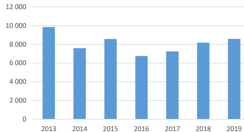
Dalsland, ack.
